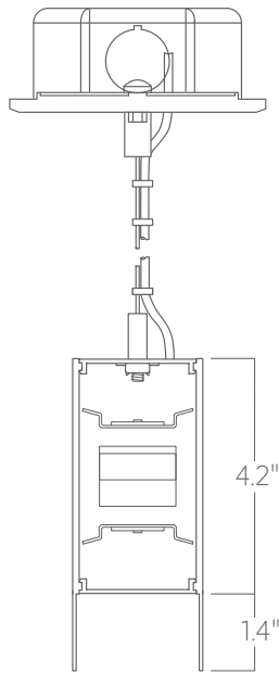
Aircraft cable 5" canopy
