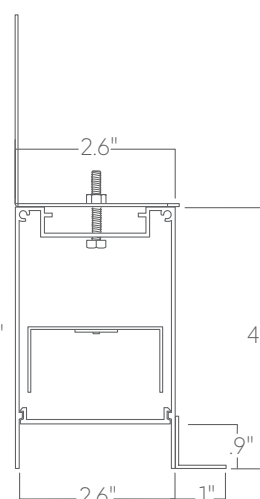
PM-F perimeter to flange
