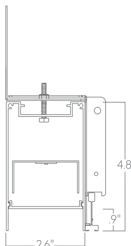
PM-SG perimeter to slot grid
