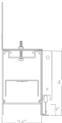
PM-T perimeter to 9/16" tee grid
