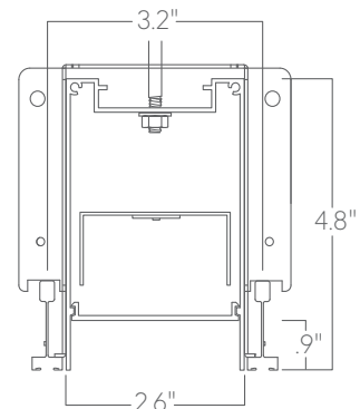
SG slot grid
