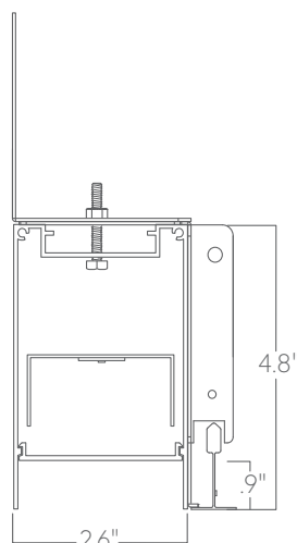
PM-T15 perimeter to 15/16" tee grid
