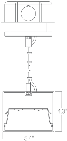
Aircraft cable 3.5" canopy
