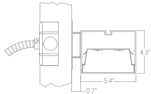
Wall mount
