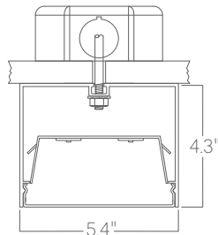
Surface mount
